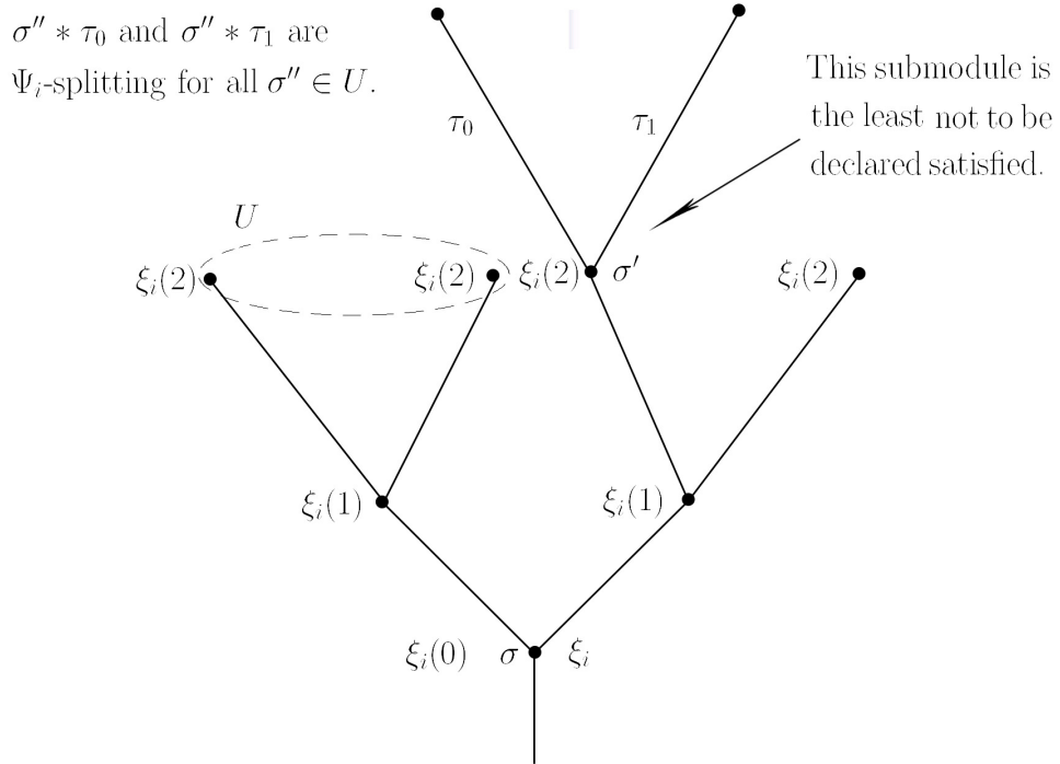
Figure 1. The placement of submodules.
